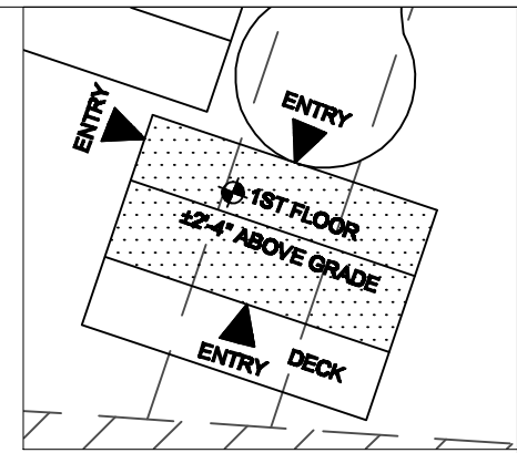
(N) HOUSE PLAN 1/32" = 1'-0"
